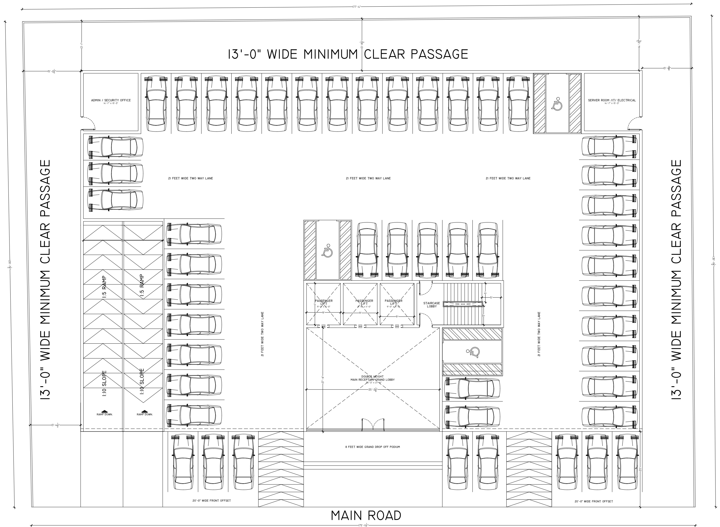
GROUND FLOOR PROPOSAL PLAN THE MERIDIAN LIVING
